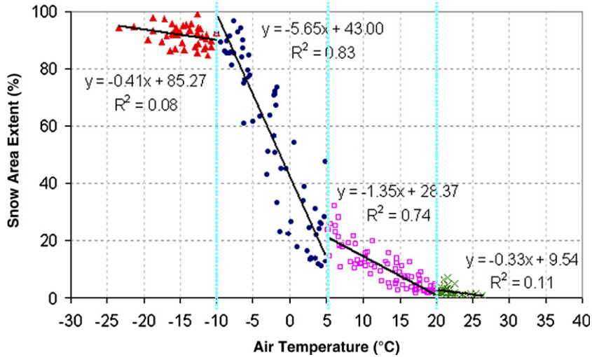
Fig. 8. Scatter plot of mean air temperature and snow area extent at different temperature ranges in the Ili River Watershed: < -10 °C, -10 °C to +5 °C, +5 °C to +20 °C, and > 20 °C.
