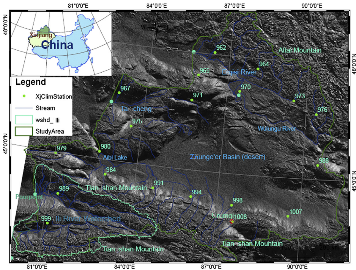
Fig. 1. Study area (green outline) of the Northern Xinjiang Uygur Autonomous Region (green region of the inset), China; cyan outline of lower left corner is the Ili River watershed; green dots are climatology stations with station ID associated; blue line stream flow network derived from 90 m SRTM DEM available at http://seamless.usgs.gov/Website/Seamless/ . Background image is the hillshaded DEM (For interpretation of the references to colour in this figure legend, the reader is referred to the web version of this article.).
