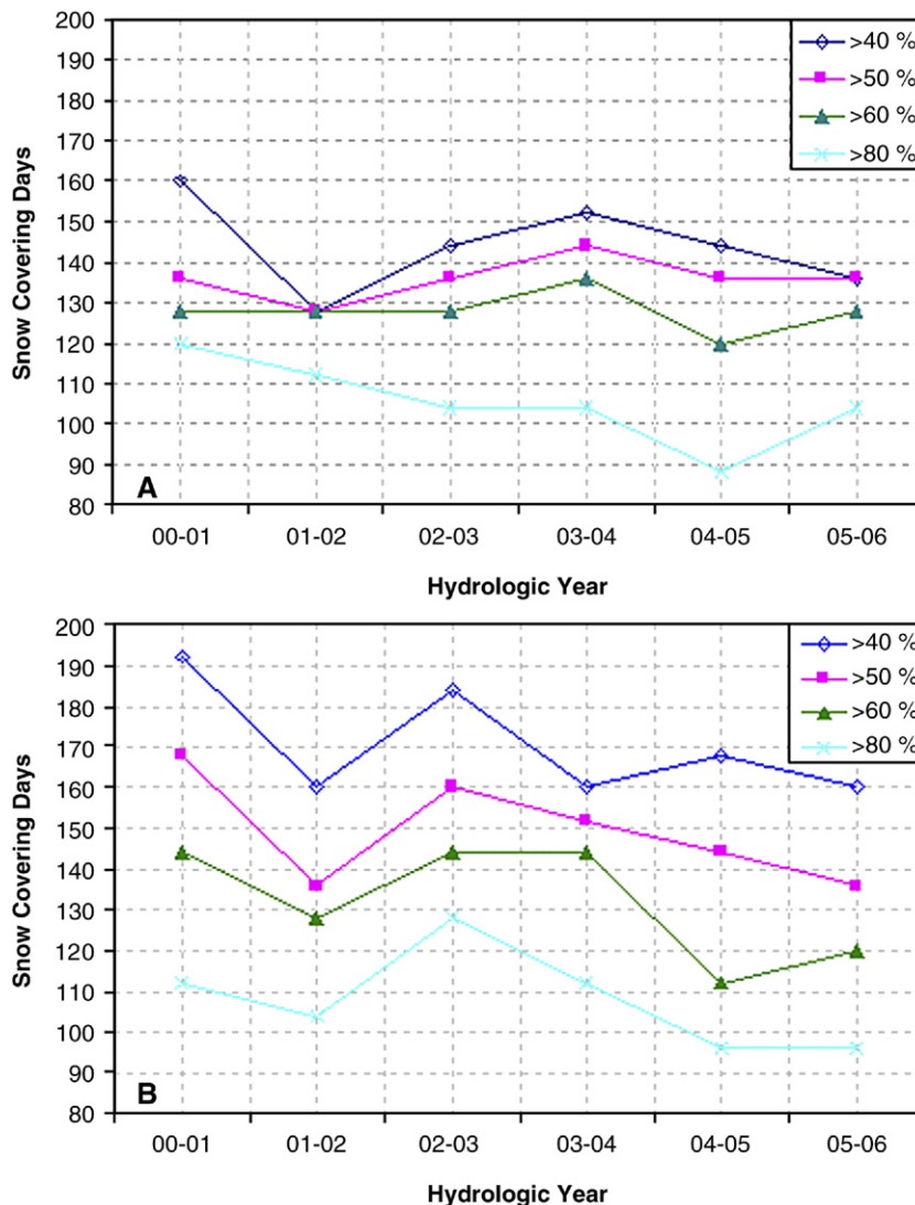
Fig. 7. Snow covered days based on different SAE thresholds at the entire Northern Xinjiang (A) and Ili River Watershed (B) vs hydrologic years of 2000–2006 period.
